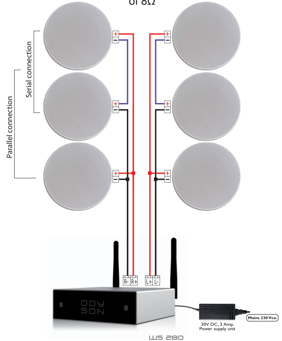
Installation with 6 Speakers of 8 \Omega
