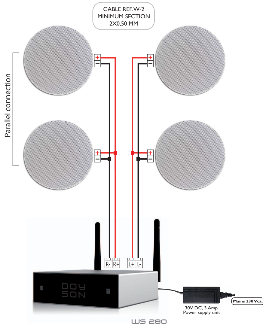
Installation with 4 Speakers of 8 \Omega
