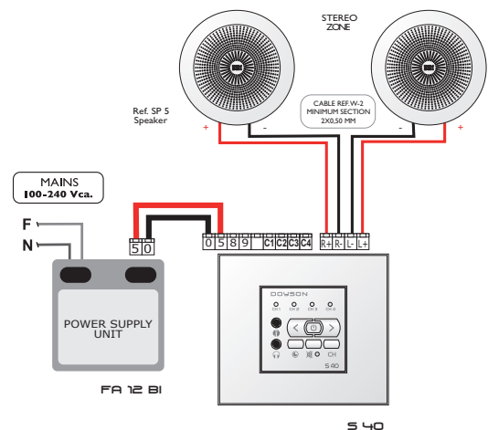
Installation diagram with power supply unit
