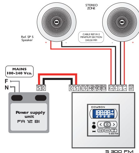
Installation diagram with power supply
