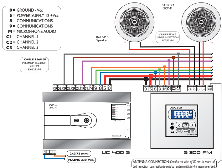
Installation diagram with Central Unit
