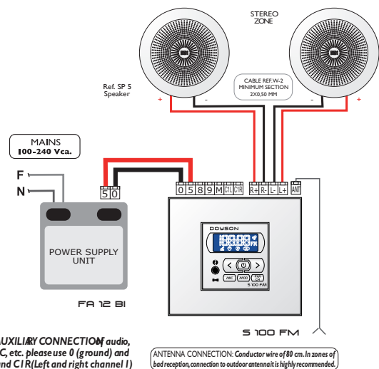
Installation diagram with power supply
