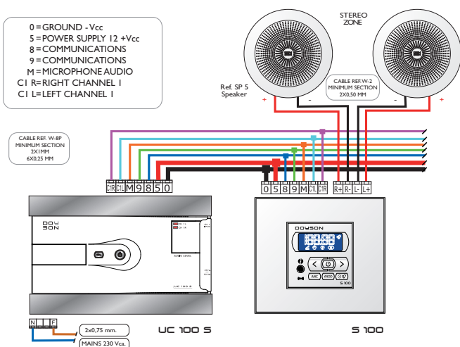
Installation diagram with Central Unit
