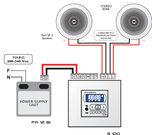
Installation diagram with power supply
